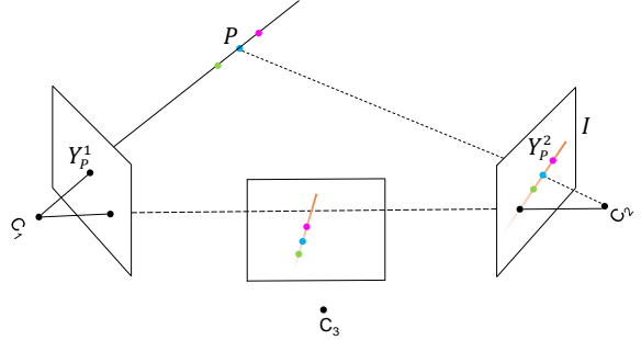
Figure 3. Geometric illustration of multi-view feature fusion. An image point Y_{\rho}^1 back-projects to a ray in 3D defined by the first camera center C_1 and Y_{\rho}^1 . This line is imaged as I in the second view. The 3D point P which projects to Y_{\rho}^1 must lie on this ray, so the image of P must lie on I . If the camera poses change, for example, we move the camera 2 to 3, then we can approximately get the corresponding line by applying an appropriate affine transformation to I . See section 3.
